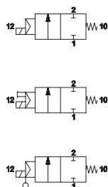
2/2 NC AF-2550 G1
